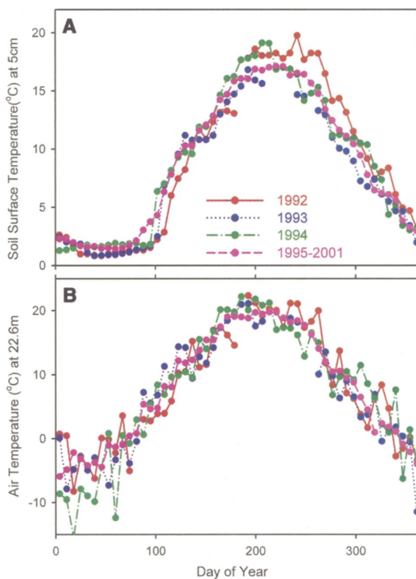
Fig. 3. Seasonal variations of the weekly mean soil surface temperature at 5 cm (A) and the air temperature at 22.6 m (B) at Harvard Forest. The average for the years from 1995 to 2001 was obtained from the hourly measurements directly (not from the average of means).
