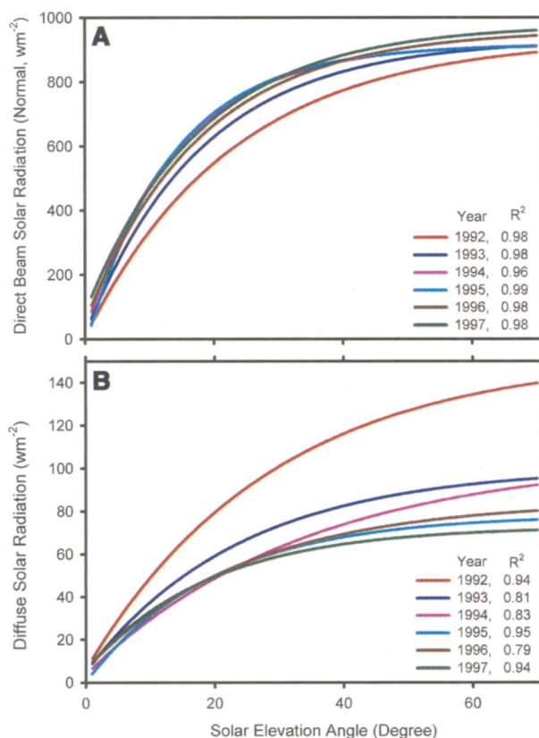
Fig. 1. Regression between the cloudless solar radiation and the solar elevation angle for the 6 years (1992 to 1997) after the Mount Pinatubo eruption. The regression relation is I = c_0 + c_1 \cdot [1 - \exp(-c_2 \cdot \theta)] . I is the direct beam or the diffuse solar radiation. c_0 , c_1 , and c_2 are regression coefficients. \theta is the solar elevation angle. Diffuse radiation and direct beam radiation were measured independently. Because of this, some minor mismatch between diffuse and direct radiation in the year-to-year variations existed, but it was not found to affect the final results considerably (SOM text; figs. S3 and S4). (A) Direct beam solar radiation on the normal plane. (B) Diffuse solar radiation.
